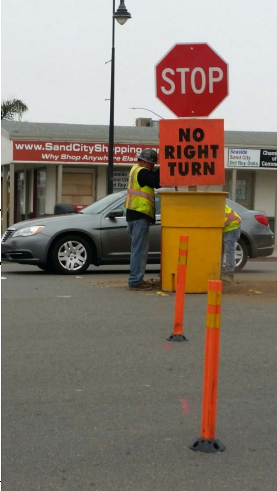
Intersection: prohibit right turn into construction work zone eastbound
