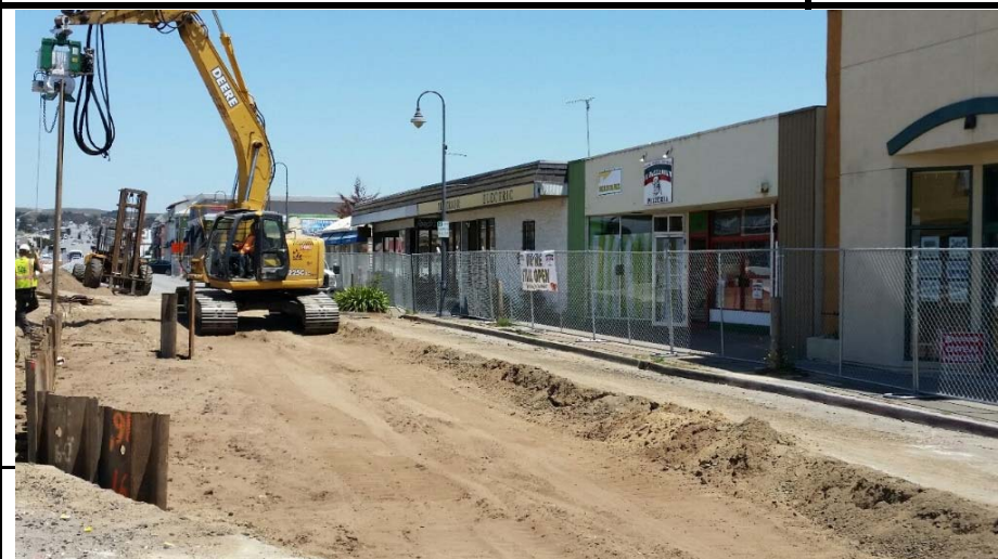
Infiltrator #3 Sheet Pile installation
